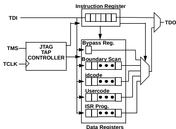
Figure 6. JTAG Interface
