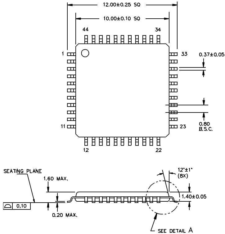
44-Lead Thin Plastic Quad Flat Pack A44
