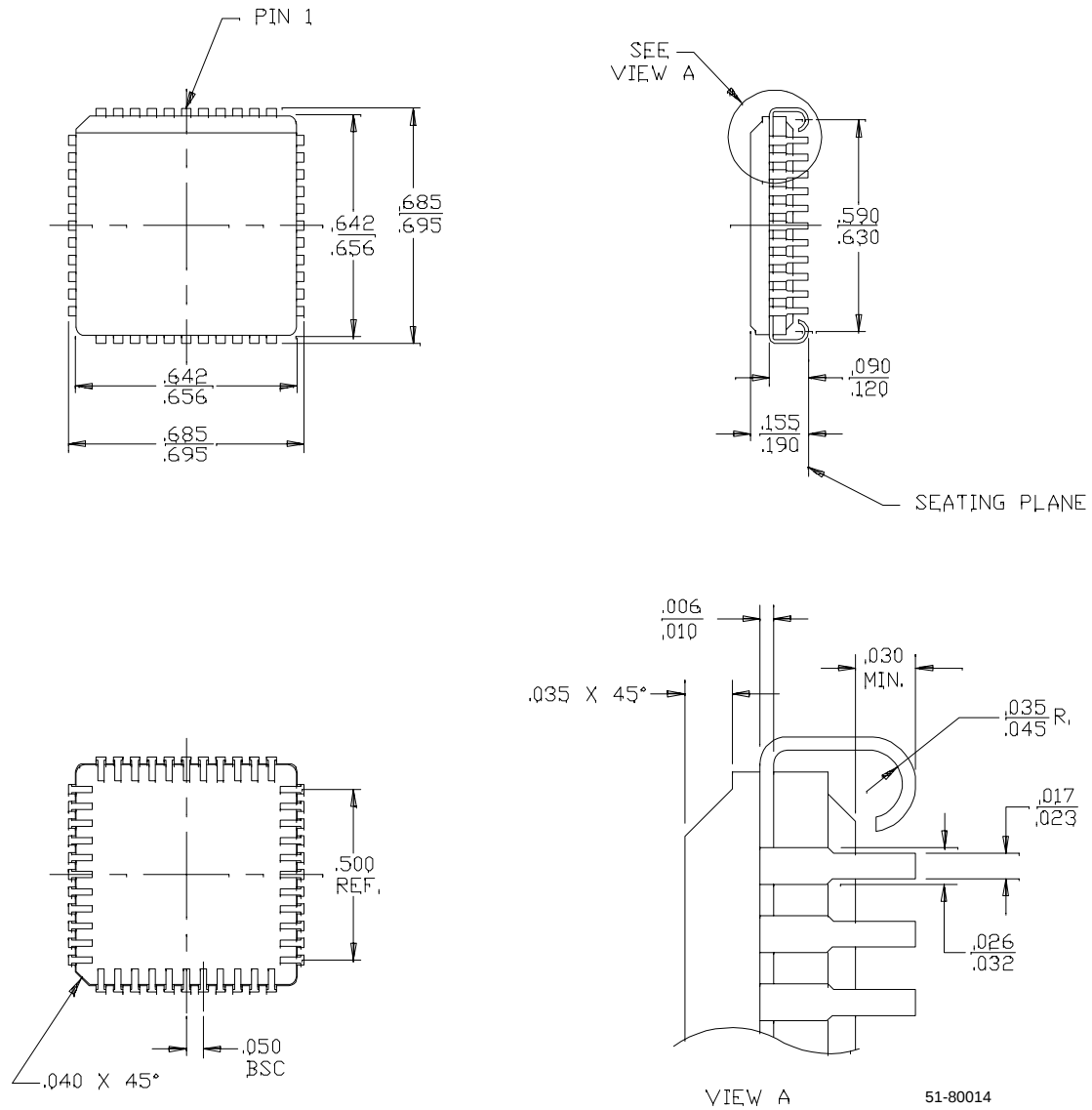
44-Pin Ceramic Leaded Chip Carrier Y67
